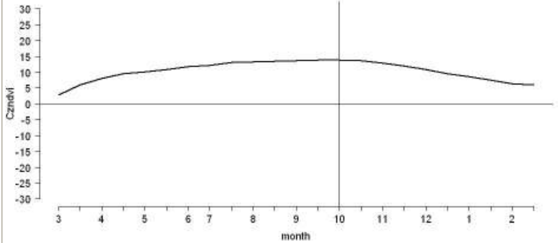
Figure 2. Czndvi in North Horr from March 2010 to February 2011
