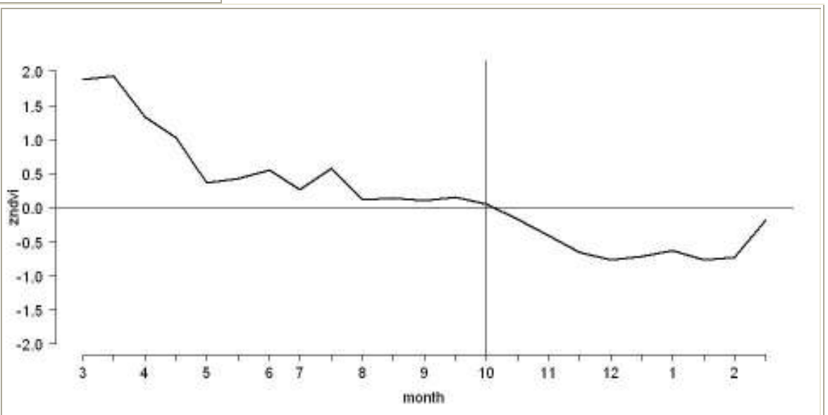
Figure 1. ZNDVI in North Horr from March 2010 to February 2011
