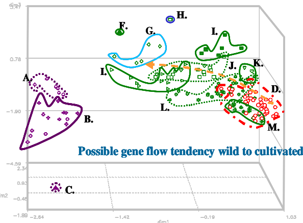
Figure 3. The population distribution with all markers using MCA. purple: cultivated type, green: weedy type and red: wild type.
