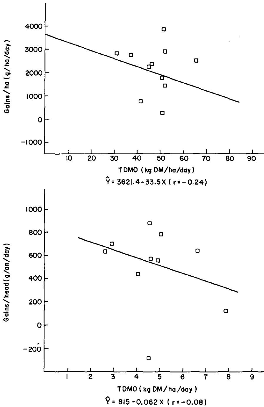
Figure 11. Relationship between animal gains per ha and per head with total DM on offer (TDMO) in a continuously grazed Andropogon gayanus 621 + Centrosema pubescens paddock.
