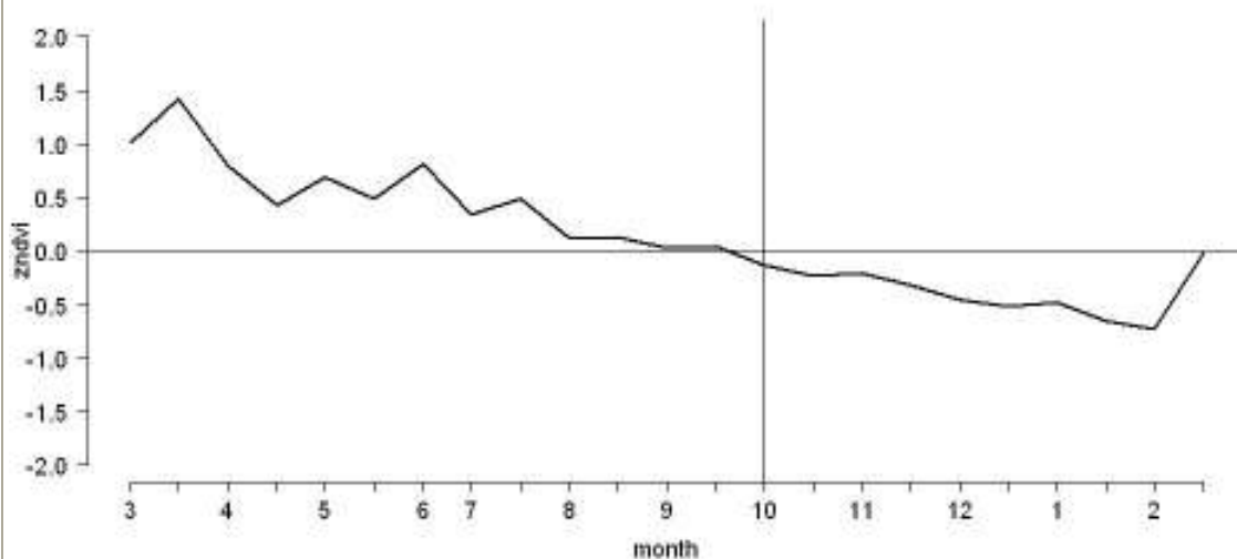
Figure 1. ZNDVI in Loiyangalani from March 2010 to February 2011
