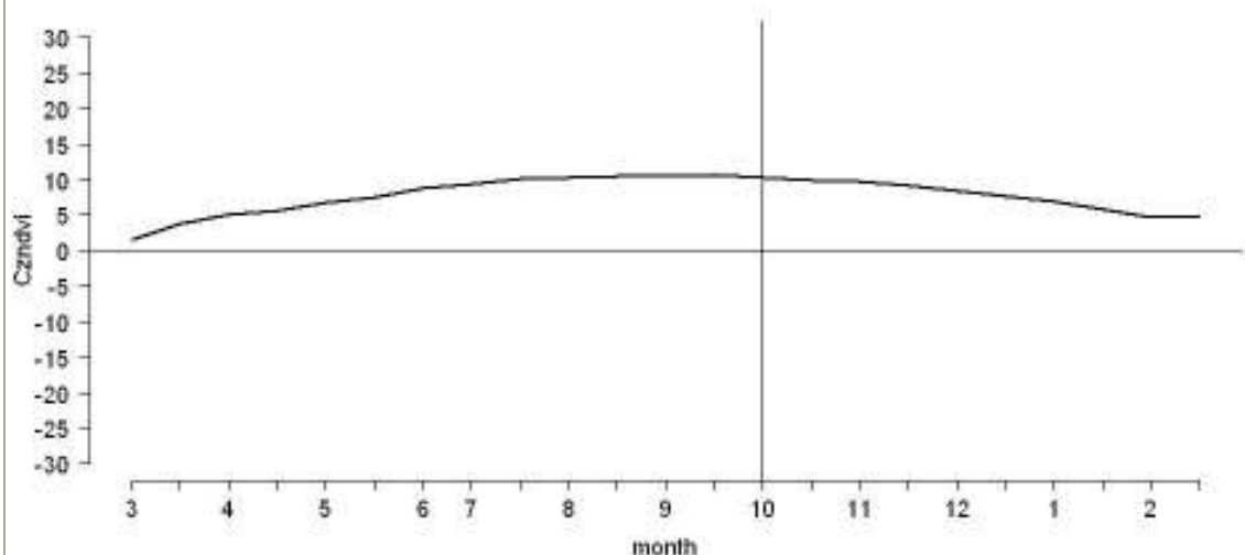
Figure 2. Czndvi in Loiyangalani from March 2010 to February 2011
