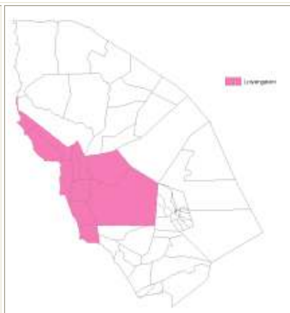
Loiyangalani
