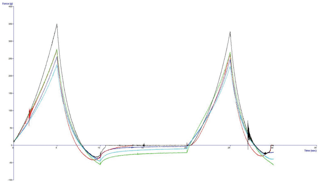
Figure 4. Instrumental texture profile analysis curve of cooked fufu dough produced from NR1741 gari.
