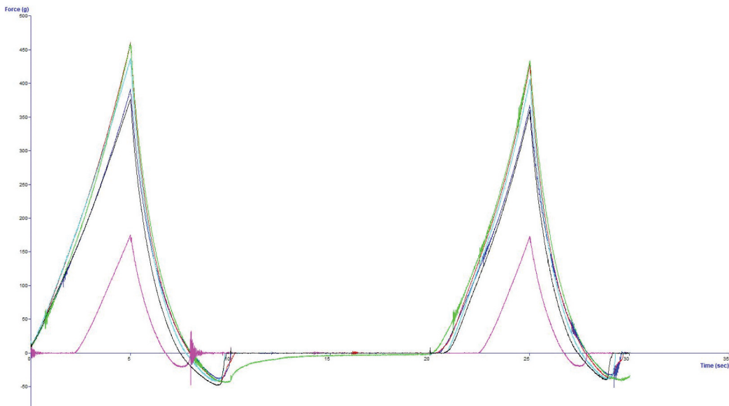
Figure 3. Instrumental texture profile analysis curve of cooked fufu dough produced from TMBE419 gari.
