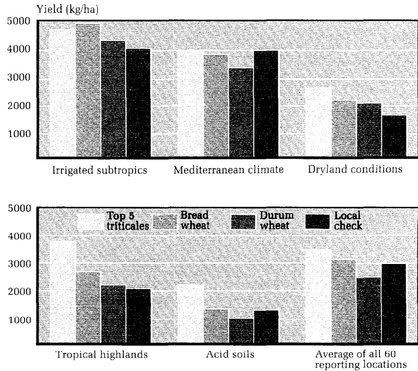
Fig. 4.1. Relative yield performance of triticales under differing agroclimatic conditions. a
