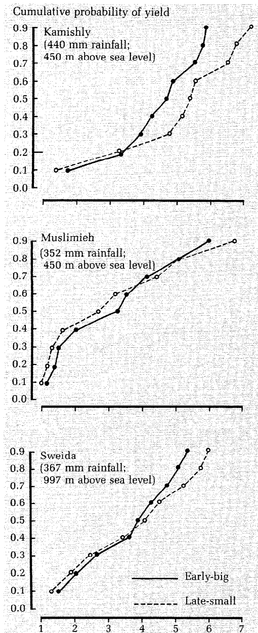
Fig. 2.2. Simulation of grain yield by two hypothetical wheat varieties at three locations in Syria. a
