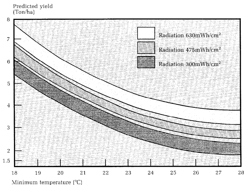
Fig. 2.1. Predicted yield for irrigated rice based on minimum temperatures and solar radiation during ripening. a
