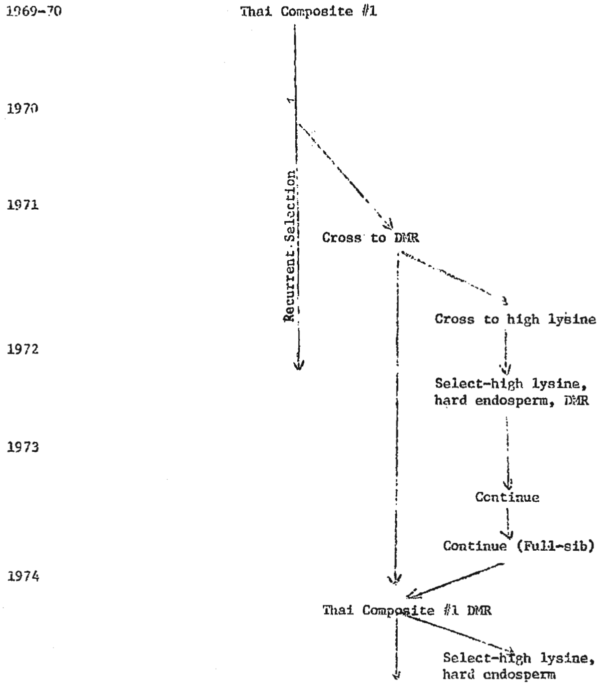
FIGURE 4 - Development of High Lysine Maize with High Yield and other Important Traits.
