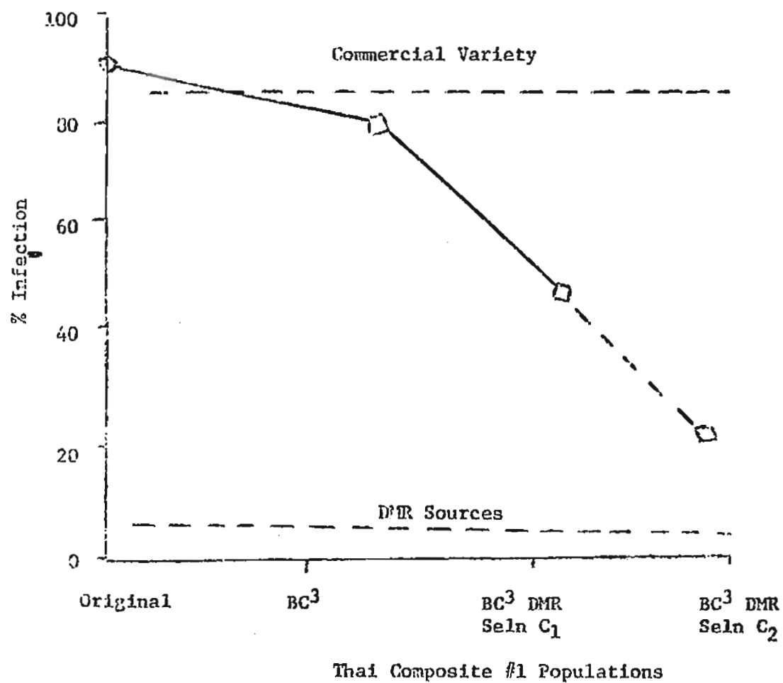
FIGURE 5 - Progress in the Transfer of Downy Mildew Resistance to Thai Composite #1.
