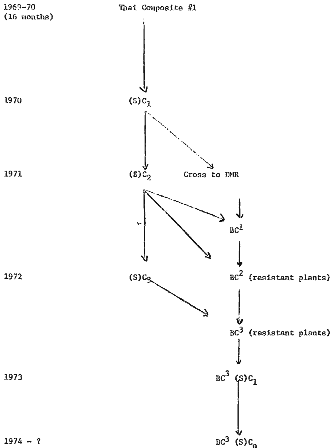
FIGURE 2 - Recurrent Selection (S 1 Progeny) for Grain Yield, Disease Resistance and Other Important Traits.
