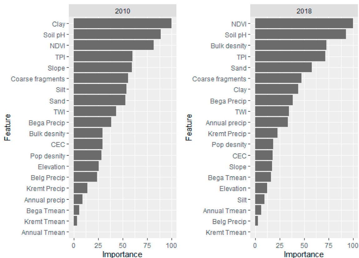
Fig. 3. Important variables for predicting SOCst in before (2010) and after (2018) SLM interventions in Ethiopia as identified based on RF model. Predictors are explained in Table 2.
