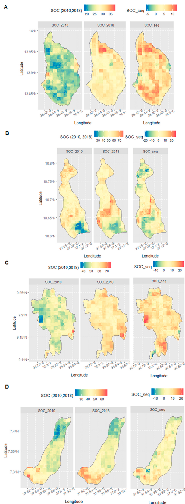
Fig. 4. Spatial distribution of SOC stocks (Mg ha -1 ) using RF model in 2010, 2018; and difference (SOC sequestration in 8 years) in the four SLMP watersheds of Ethiopia: A) Adi Tsegora, B) Yesir, C) Gafera, D) Azuga shuba watershed.
