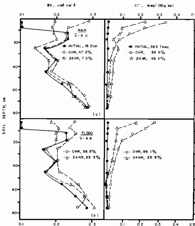
Fig. 24. Water content, \theta_v and chloride, \text{Cl}^- , distributions with depth for different redistribution times (in hr) in soil under conventional tillage at \theta_i = 0.195 \text{ cm}^3 \text{ cm}^{-3} . Five cm of 0.02N \text{CaU} solution was added as (a) rain, and (b) flood; \bar{v} represents average infiltration rate in \text{cm hr}^{-1} .
