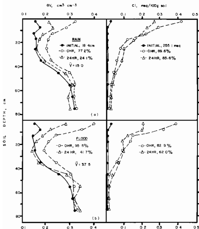
Fig. 23. Water content, \theta_v and chloride, \text{Cl}^- , distributions with depth for different redistribution times (in hr) in soil under zero tillage at \theta_i = \theta_a = 0.216 \text{ cm}^3 \text{ cm}^{-3} . Five cm of 0.02N \text{Ca U}_2 solution was added as (a) rain, and (b) flood; \bar{v} represents average infiltration rate in \text{cm hr}^{-1} .
