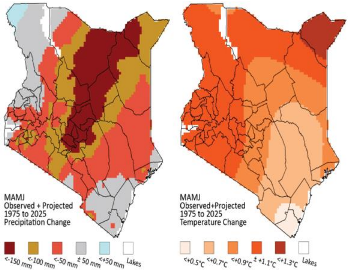
Figure 1: Observed and projected changes in precipitation and temperature in Kenya (1975, 2025). Source: USAID, 2010
