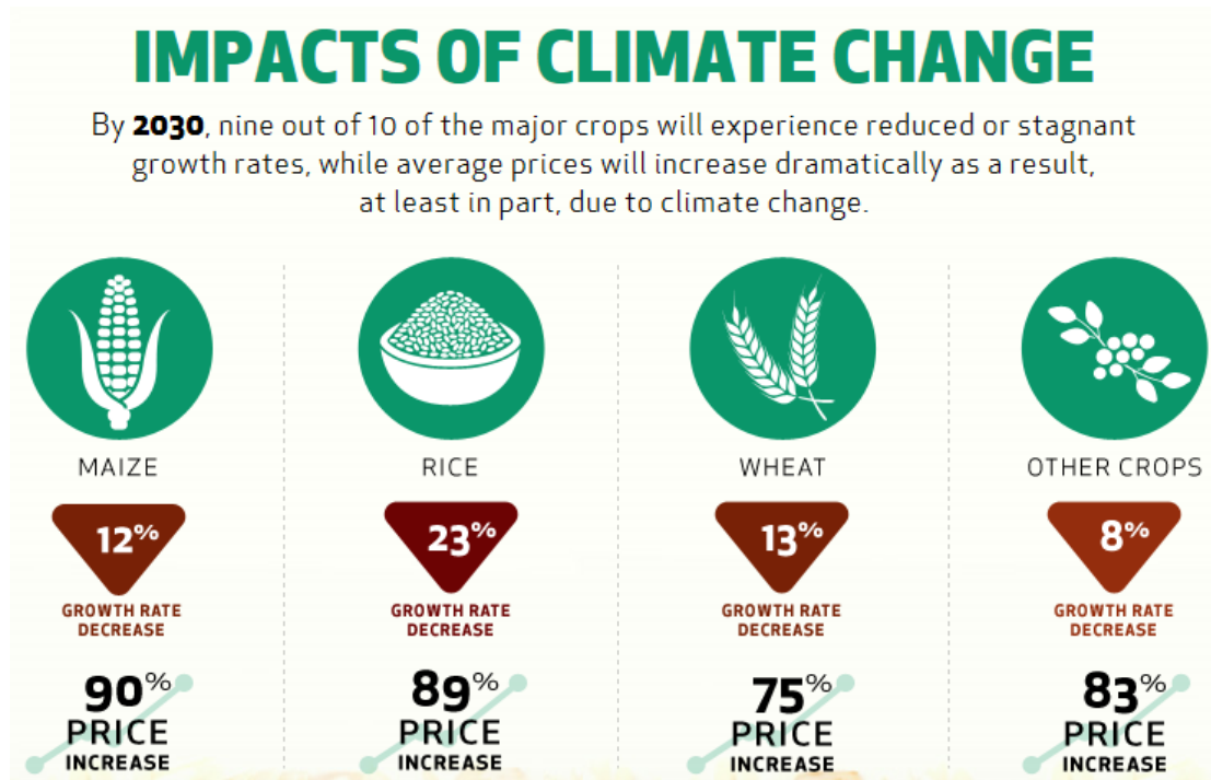
Figure 2: Projected impacts of climate change on main crops in Kenya by 2030. Source: Tegemeo Institute (2010),
