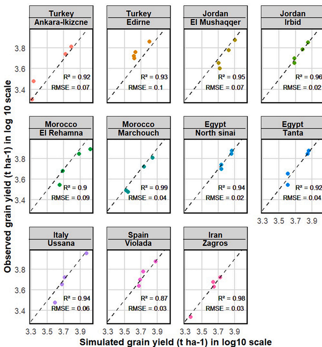
Fig. 3. Calibration and evaluation of the model using baseline \log_{10} -transformed grain yield ( \text{t ha}^{-1} ) for 11 sites of 7 Mediterranean countries. Observed vs. simulated grain yields are plotted, values inside the figures are Root Mean Square Error (RMSE) and Pearson coefficient of determination ( R^2 ) for each site.
