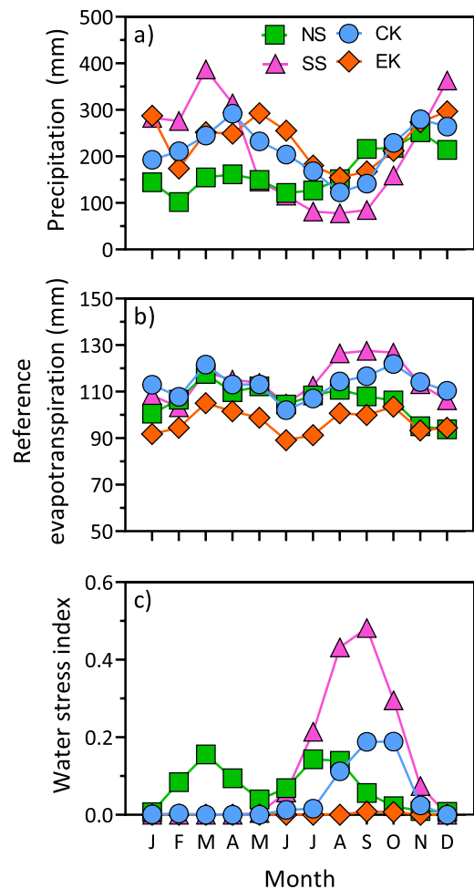
Fig. 4. Annual patterns in (a) monthly precipitation, (b) reference evapotranspiration (ETo), and (c) water stress index for the four regions: Northern Sumatra (NS), Southern Sumatra (SS), Central Kalimantan (CK), and Eastern Kalimantan (EK). Data are averages for all blocks within a region. Description of the methodology used to estimate ETo and water stress index is provided in Section 2.2.
