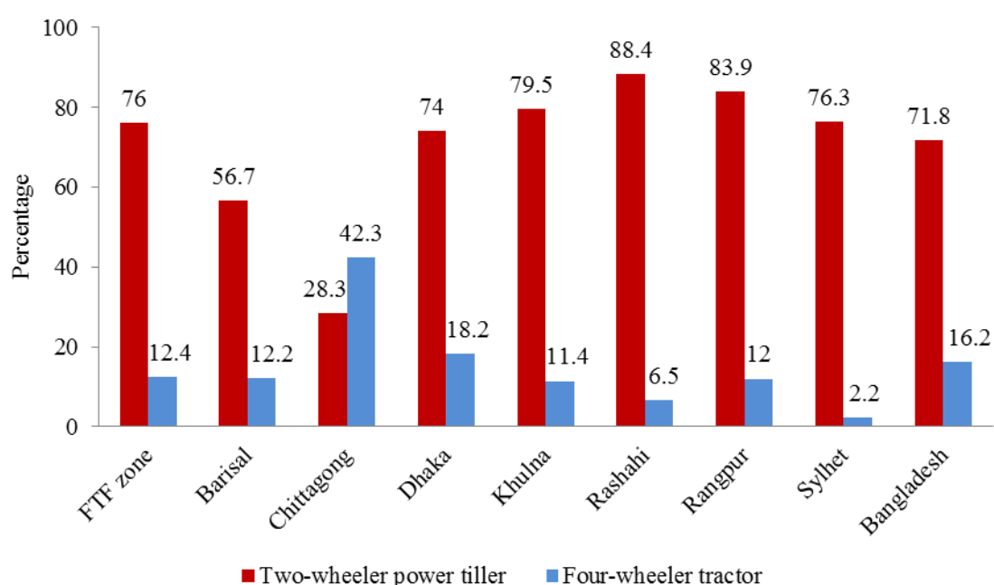
Figure 4.19—Percentage of farmers using machines for land preparation
