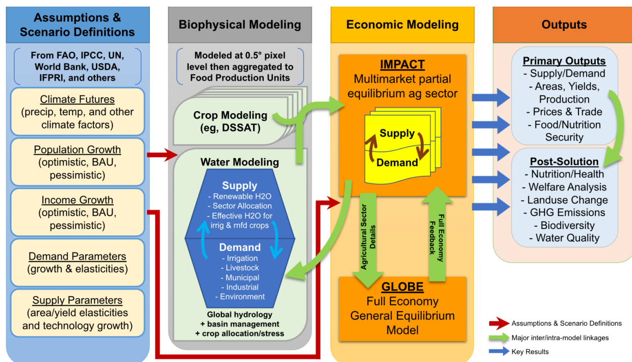
Figure 2.1.1 The IMPACT-GLOBE modeling system
