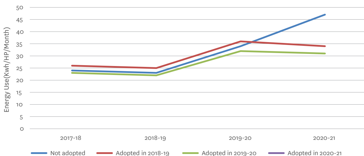
Figure 2b. Energy used for groundwater extraction (kWh/hp/month), dry period (January–June)
