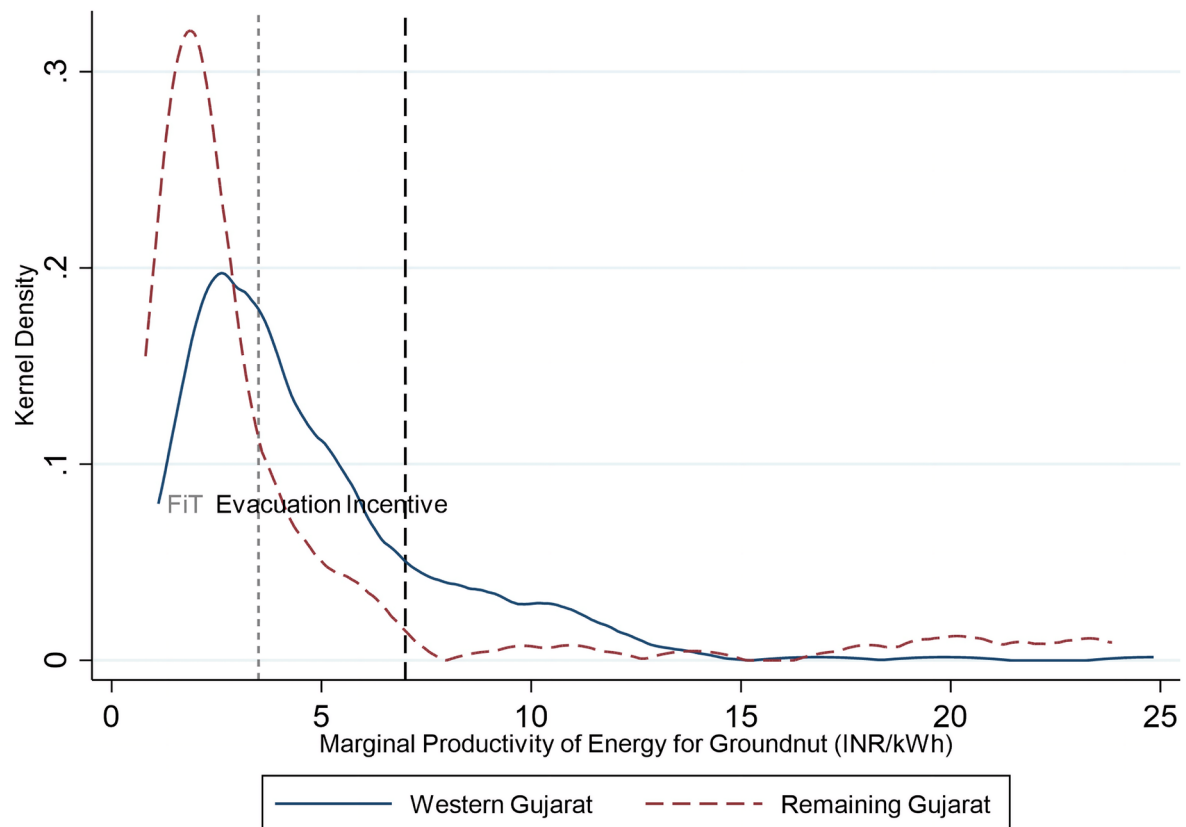
Figure 4b. Marginal returns INR/kWh for groundnut, western Gujarat
