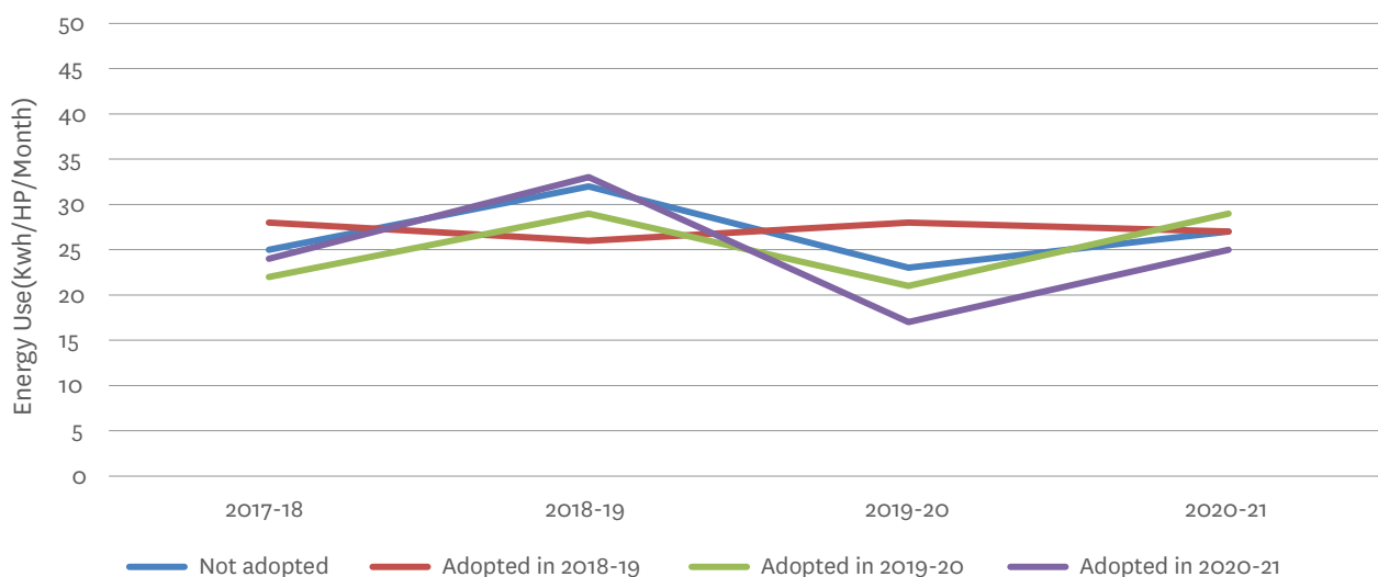
Figure 2c. Energy used for groundwater extraction (kWh/hp/month), wet period (July–December)
