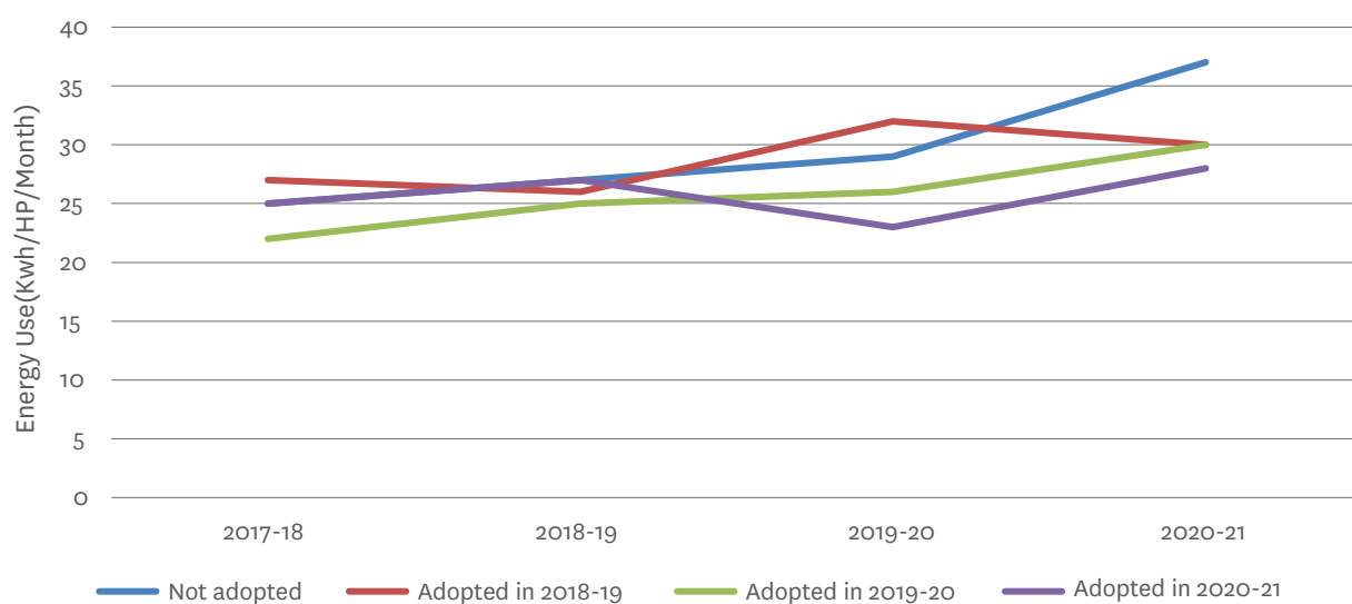
Figure 2a. Energy used for groundwater extraction (kWh/hp/month), annual period (July–June)
