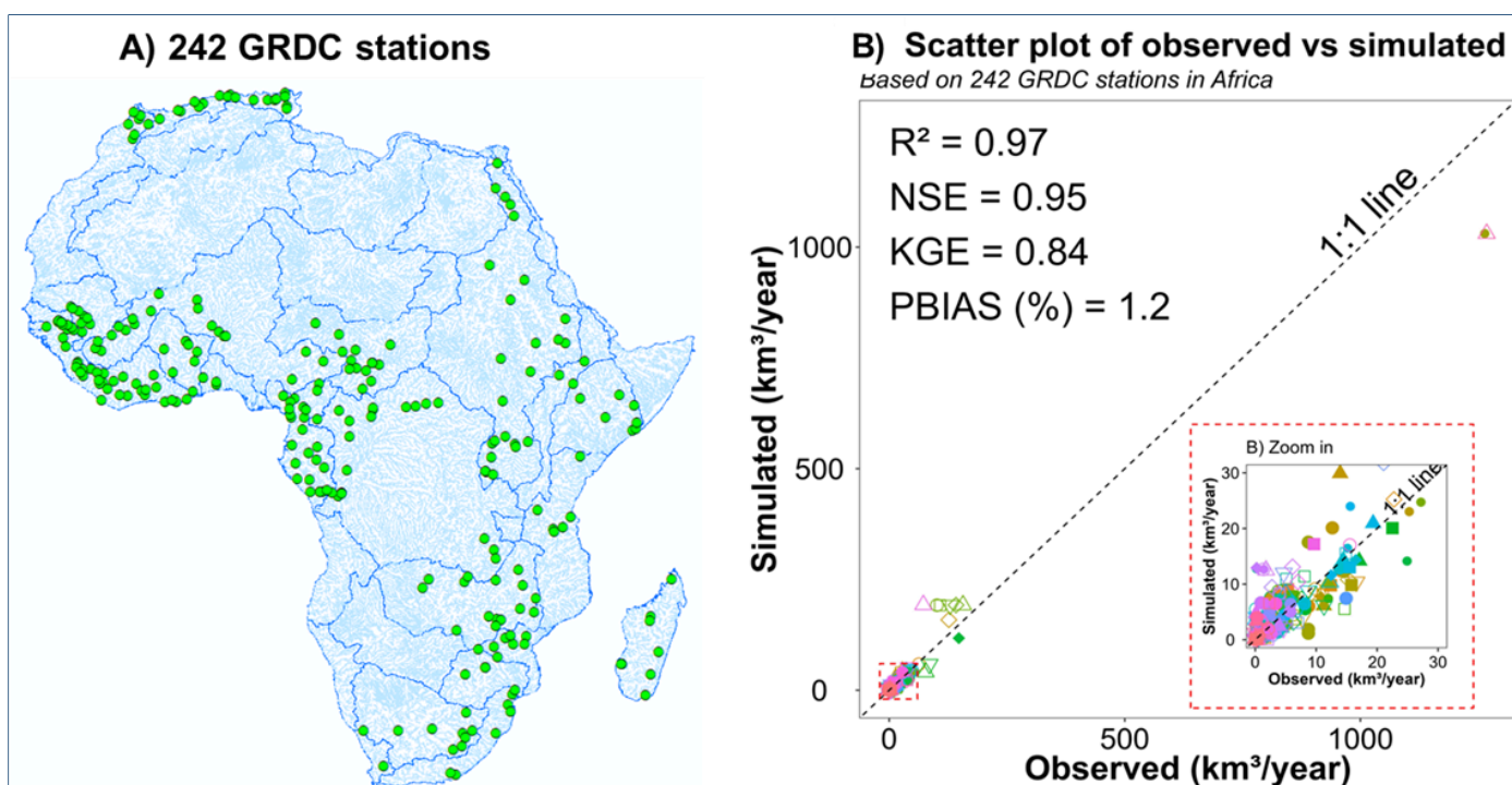
Figure 1. Comprehensive validation of the VegDischarge v1 across Africa Using GRDC data (Akpoti et al., 2024). This Figure contrasts observed annual total discharge data from 242 GRDC stations with simulated values from the VegET/mizuRoute model, reflecting the model's high accuracy in replicating discharge across varying hydrological contexts and time frames within the African continent. The inset (B) zooms in on stations with lower discharge volumes, ensuring a granular analysis of model performance in smaller basins.
