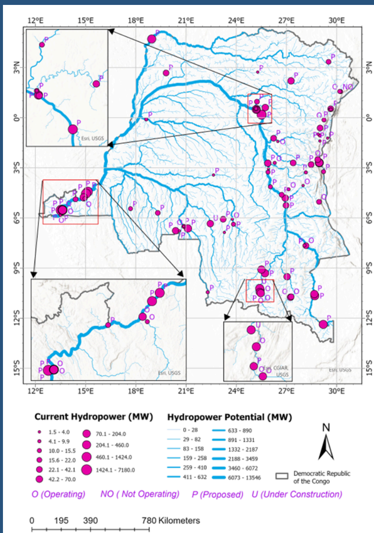
Figure 3. Indicative hydropower potential (MW) by river segment in for DRC Congo, computed from VegDischarge v1 long-term mean discharge (2000–2021) using screening parameters of 50 m hydraulic head and 0.85 turbine efficiency; segments are grouped into potential classes and shown alongside an infrastructure inventory (operational, not operational, proposed, under construction)-- infrastructure status data derived from the RePP Africa geodatabase (Peters et al., 2023).
