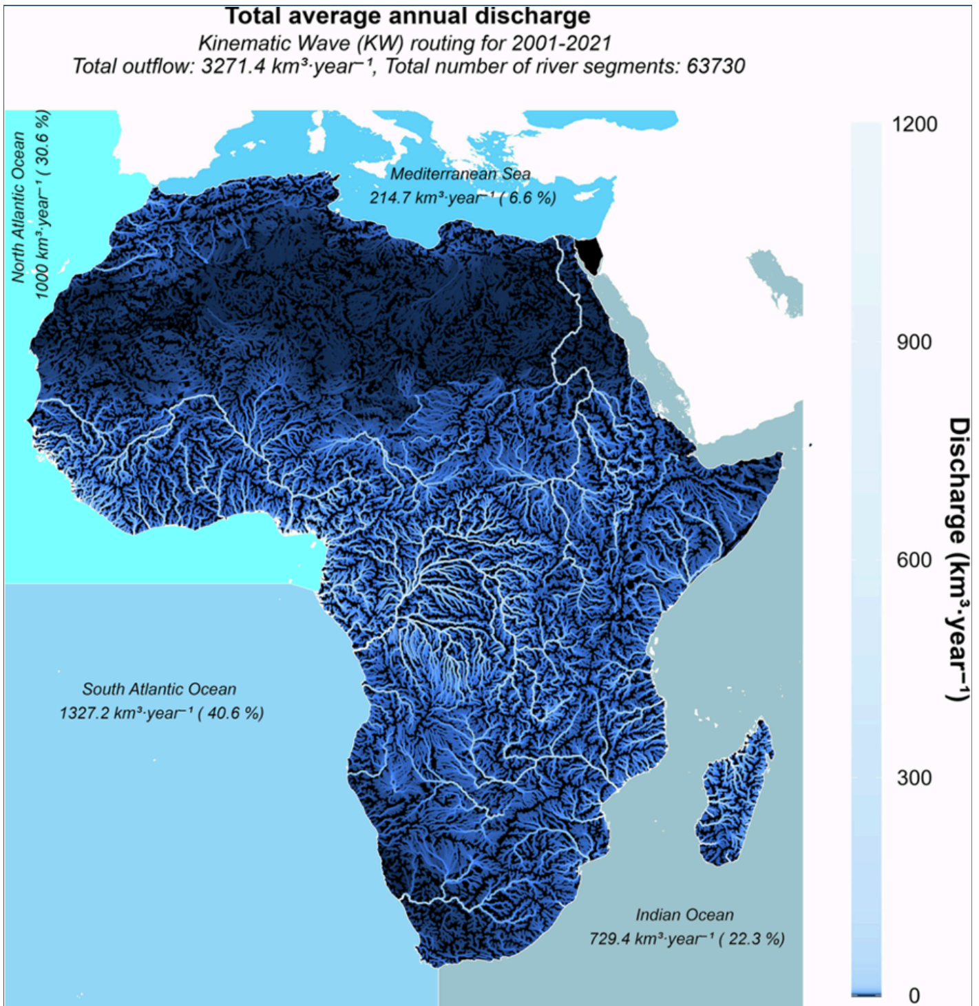
Figure 2. Total annual average discharge from Africa to adjacent oceans (2001-2021) (Akpoti et al., 2024). This map delineates the discharge of African rivers into the Mediterranean Sea, South Atlantic Ocean, and Indian Ocean, revealing the proportional contributions of each basin to the adjacent marine environments. The predominant outflow to the South Atlantic Ocean is contrasted with the lesser, yet significant, discharges into the Mediterranean and Indian Oceans.
