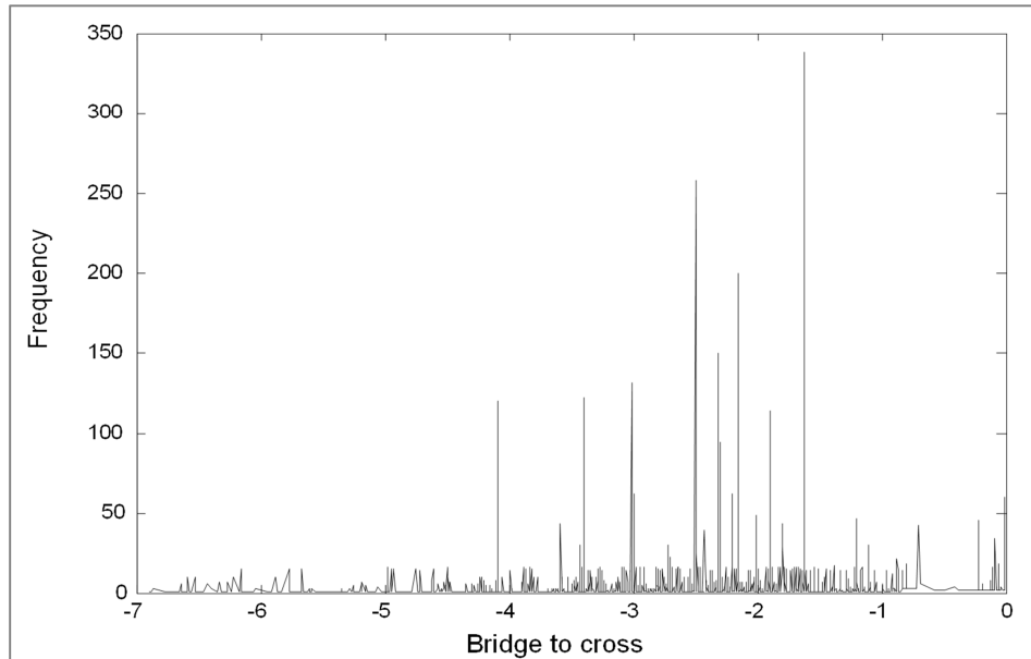
Figure 1: Distribution of \log(\text{BTC})
