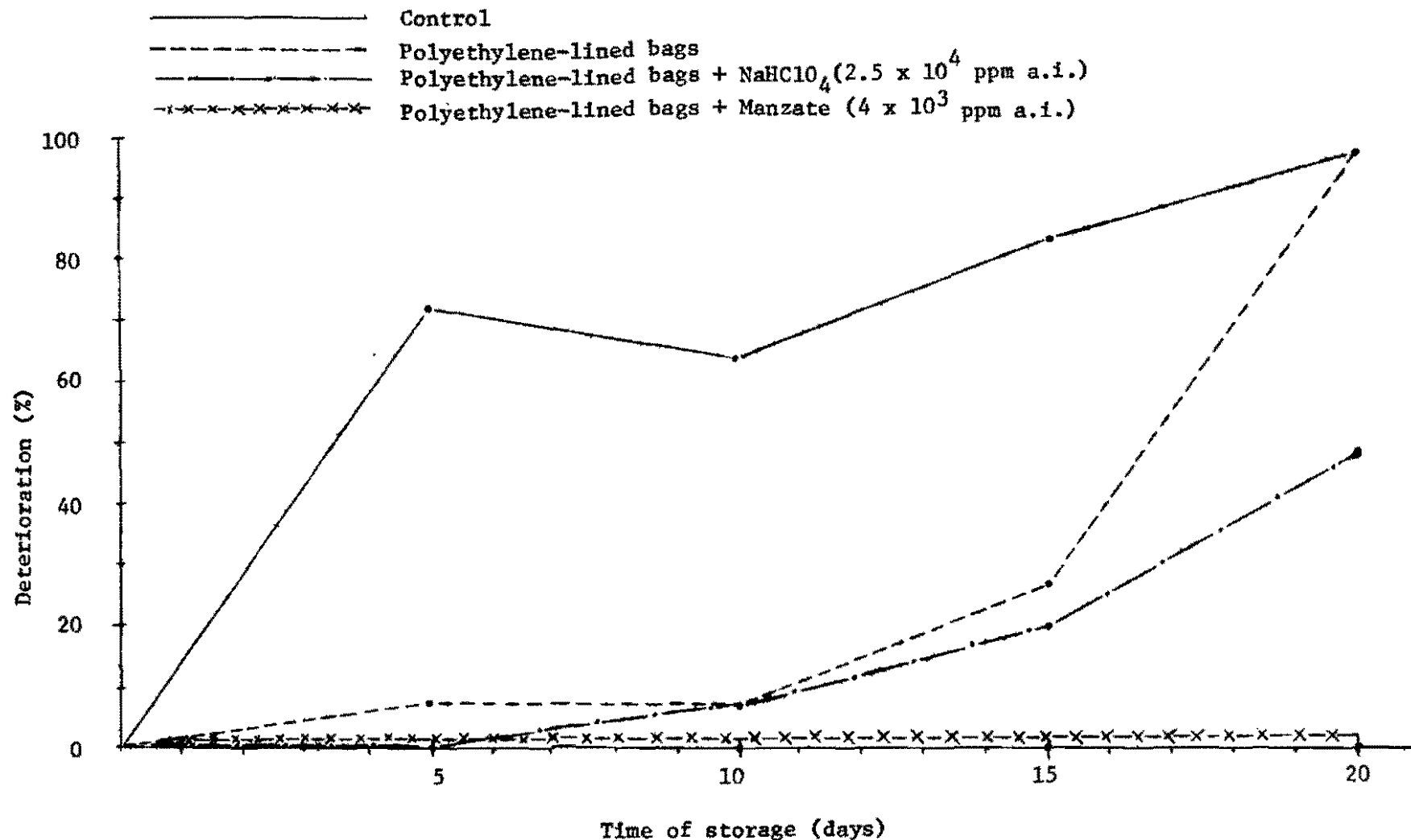
Figure 8. Effects of polyethylene-lined paper bags and chemical treatments on deterioration of stored roots.
