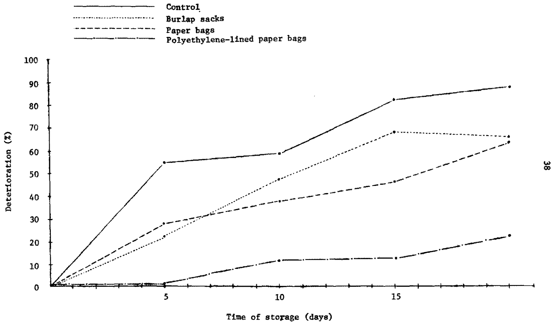
Figure 7. Effect of storage in bags on cassava (var. M.Col 113) root deterioration.
