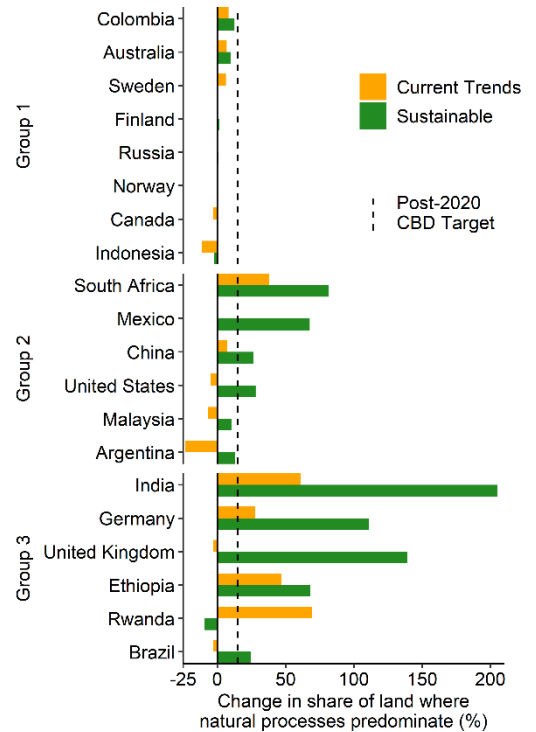
Figure 5. Modelled percentage changes in LNPP, compared to 2010
