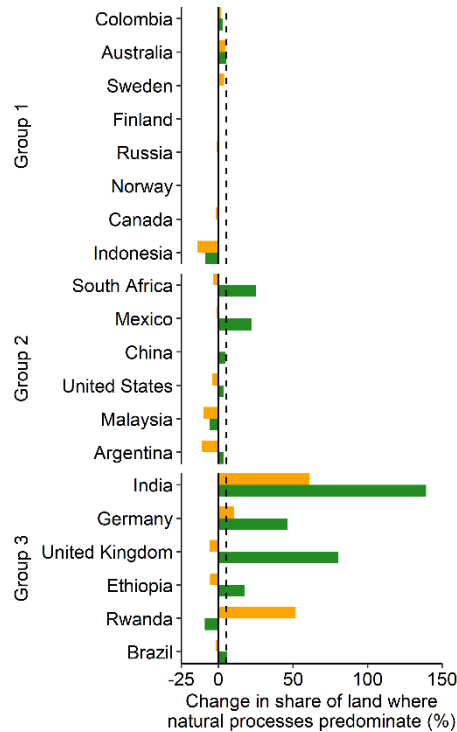
Figure 5. Modelled percentage changes in LNPP, compared to 2010
