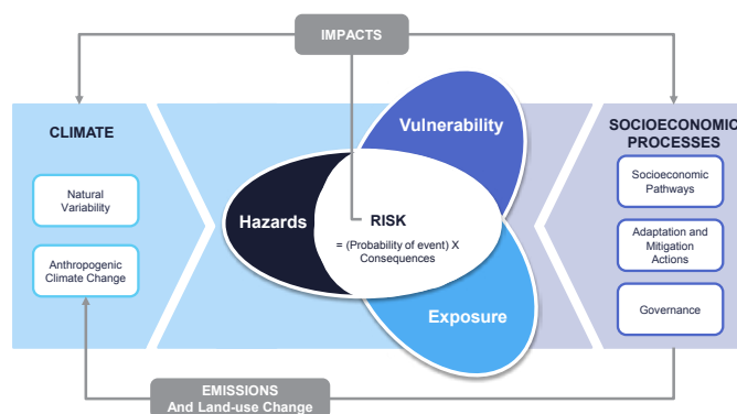
Figure 2. Schematic of the interaction among the physical climate system, exposure and vulnerability producing risk (Illustrative Example). Source: IPCC (2014)
