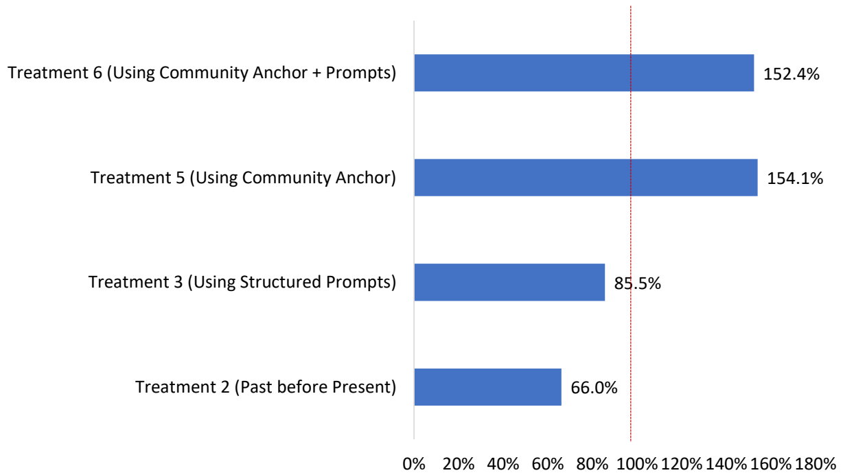
Figure 4. Extent of bias reduction in maize reports for different Treatment survey modules, relative to Treatment 1
