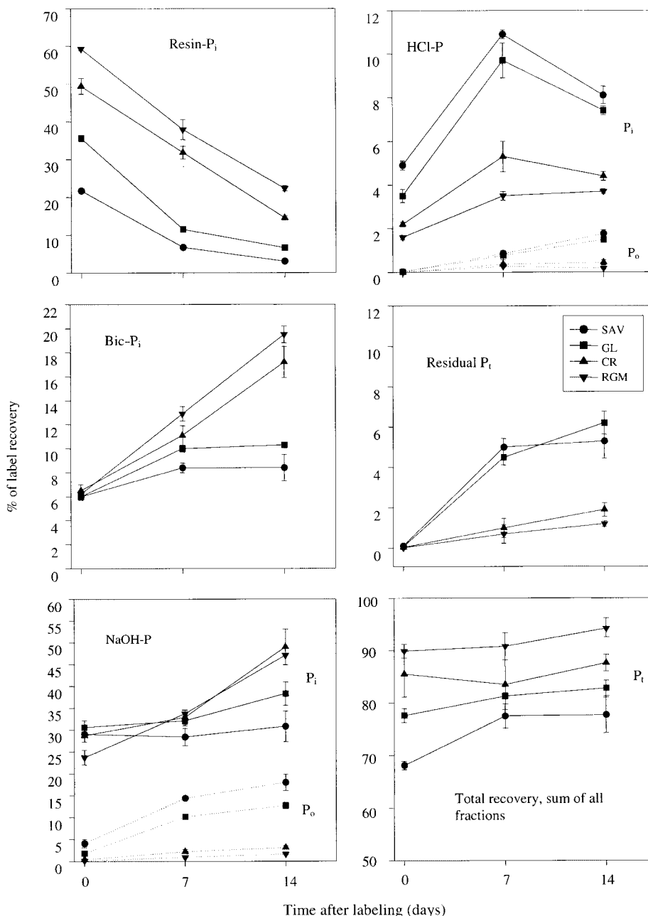
Fig. 1. Percentage of label recovery in the different fractions of the sequential P extraction and in the sum of all fractions at 4 h, 1, and 2 wk after labeling soil. Recovery in Bic- \text{P}_o in all soils at all sampling times <1% (means of three replicates \pm SD).
