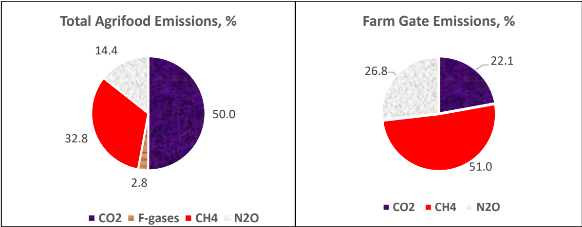
Figure 3. Agrifood Emissions by type of GHG gas in 2020, %
