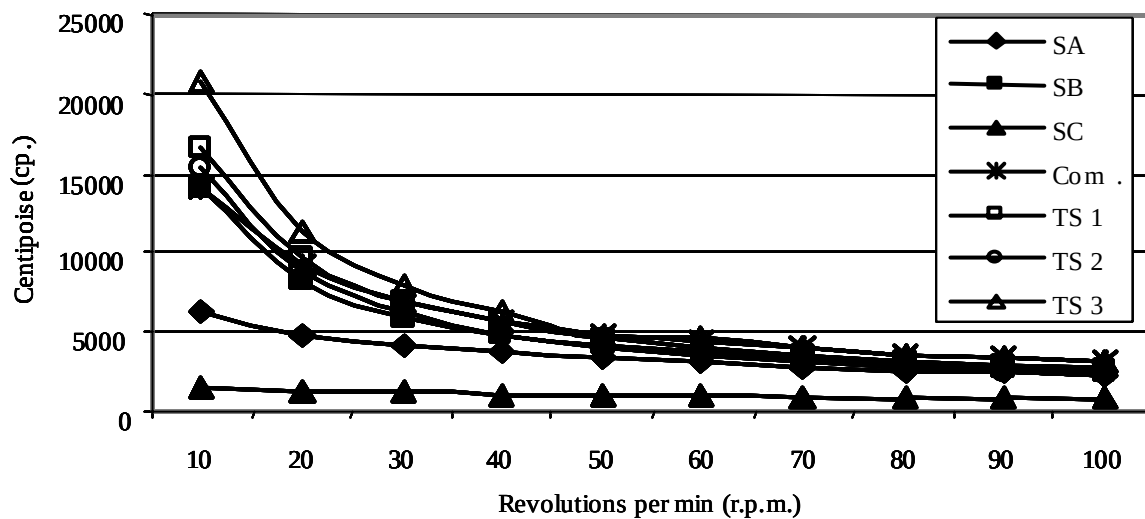
Figure 5. Viscosity of laboratory-prepared and commercial tomato sauces at room temperature.
