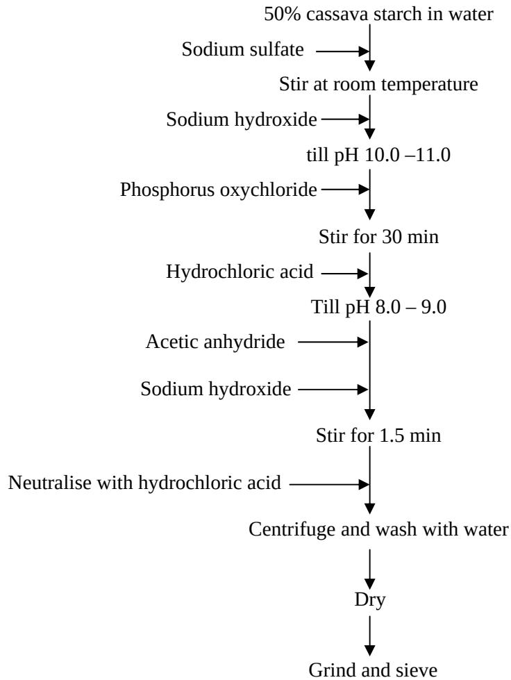
Figure 3: Preparation of cross-linked acetylated cassava starch.
