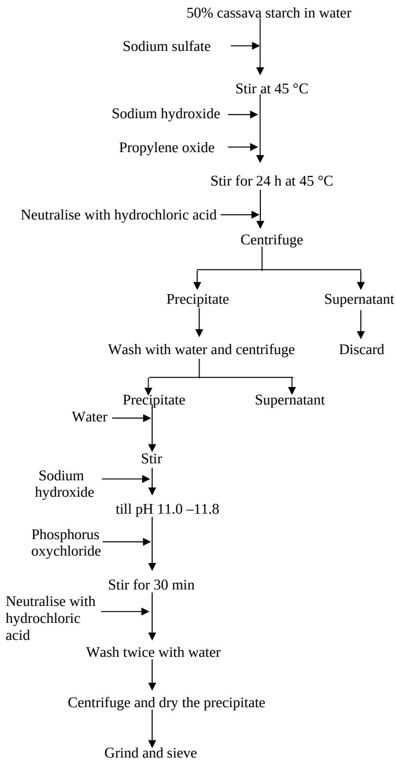
Figure 2: Preparation of cross-linked hydroxypropyl cassava starch.
