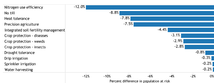
Figure 2. Change in the number of people at risk of hunger in 2050, alternative technologies, compared with the baseline.
