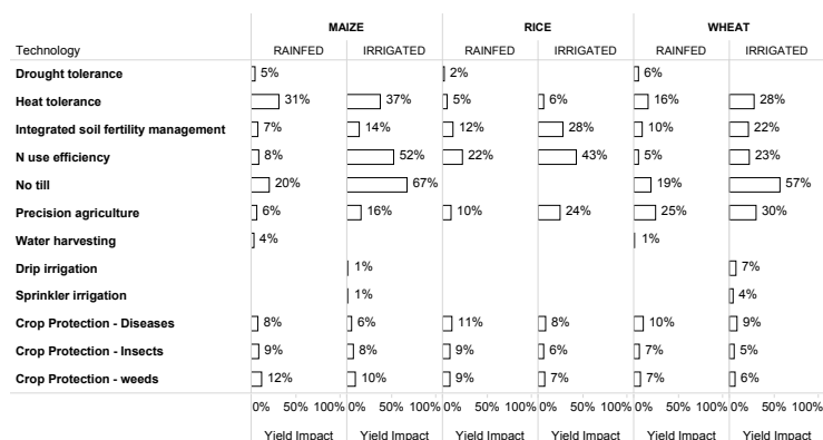
Figure 1. Global yield changes in 2050, alternative technologies, compared with the baseline (DSSAT runs).
