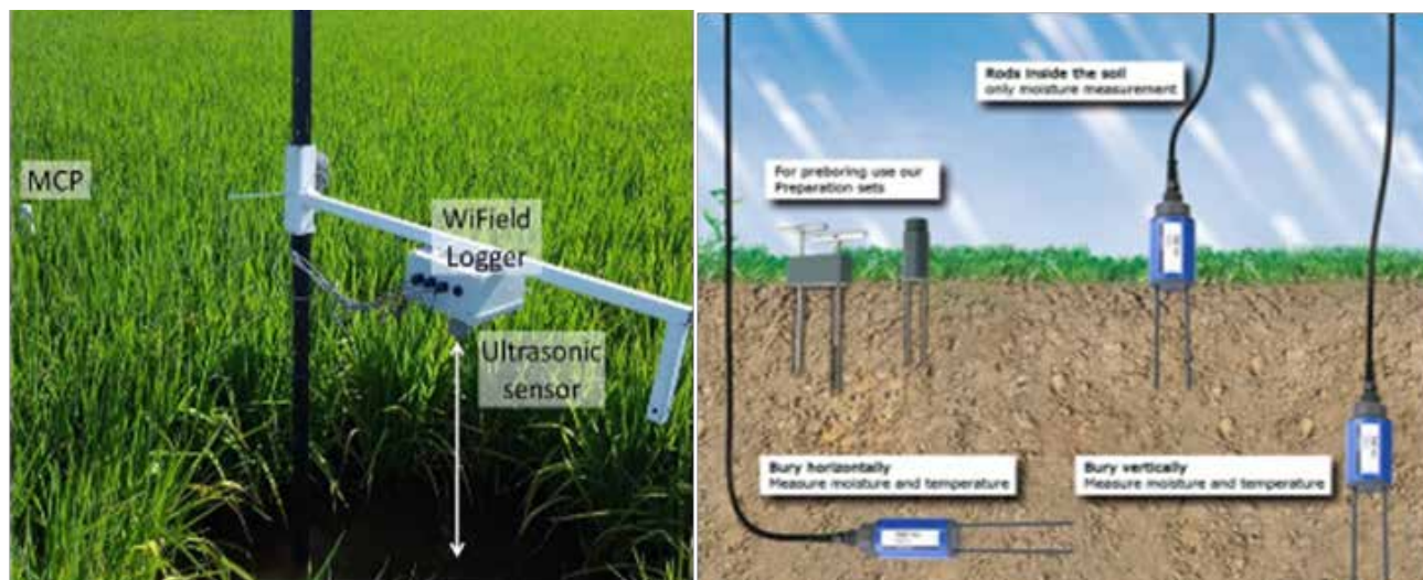
Figure 7.5. Soil Moisture Measurement using TDR
