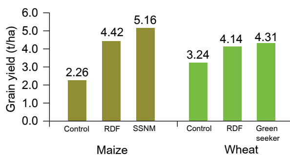
Figure 4.2. Effect of nutrient-management practices on grain yield of maize and wheat under CA
