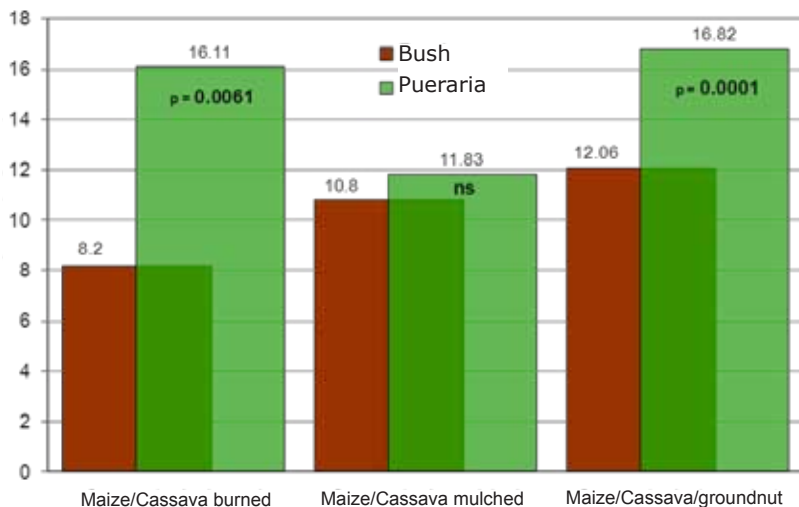
Figure 3. Cassava fresh root yield in burned and mulched maize/cassava and burned maize/cassava/groundnut intercrop after two years of natural bush or Pueraria phaseoloides fallow. On-farm, southern Cameroon, 2010-2011 (Source: Hauser, unpublished)
