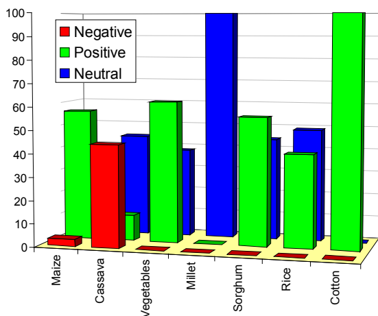
Figure 2. Crop yield response to planted herbaceous fallow in West and Central Africa. Compilation of 396 comparisons from published experiments. Source: Hauser et al. (2006).
