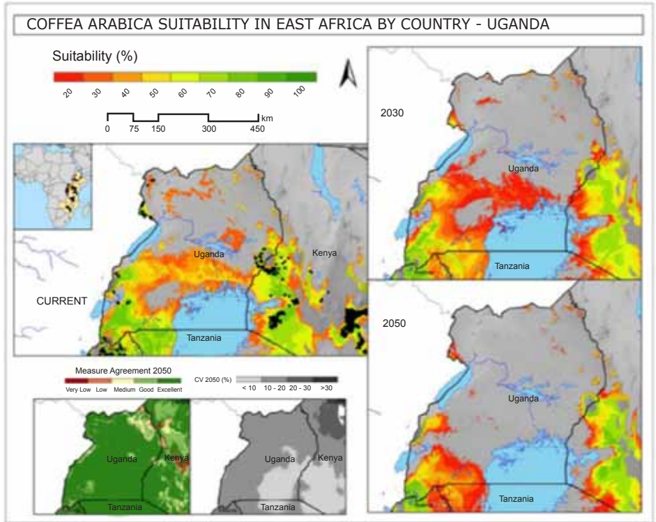
Figure 1. Change of suitability for Arabica-growing areas in Uganda using the MAXENT approach and based on a 'business as usual' climate change scenario.
