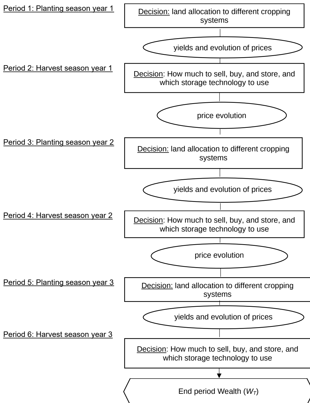
Figure 3.1 Generic discrete stochastic programming model timeline
