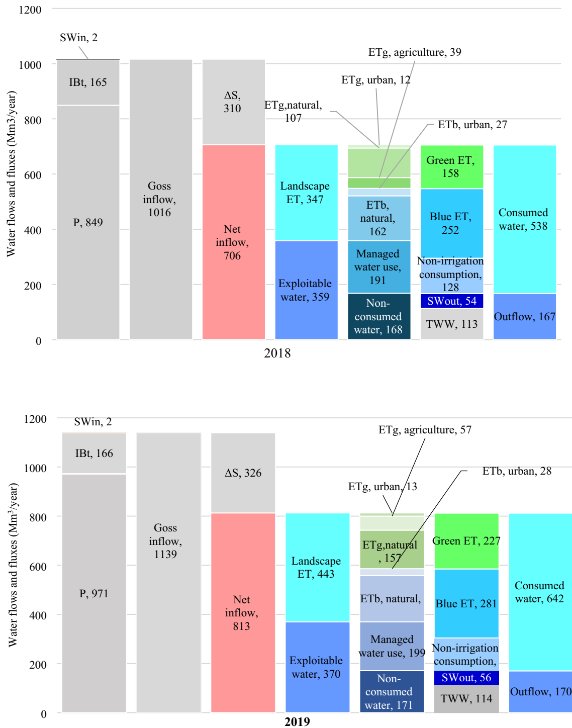
Fig. 10 The AZ basin's modified resource base sheets 2018–2021 in Mm³/year
