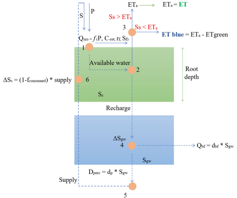
Fig. 6 Illustrative description of PixSWAB (after Michailovsky et al. 2020)
