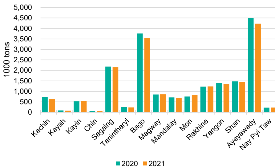
Figure 9: Paddy rice production during the monsoon of 2021
