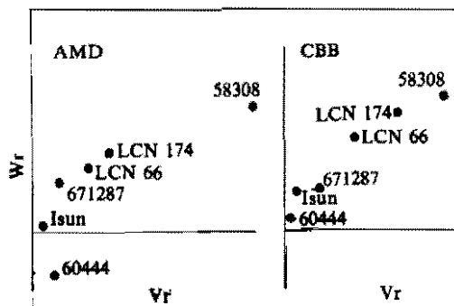
Figure 3. W_r/V_r analyses for resistance to AMD and CBB in the 6 x 6 diallel recorded at IITA. 58308 is a resistant hybrid of M. glaziovii origin; LCN 174 and LCN 66 are selections from the cross 58308 x Isunikakiyan; Isunikakiyan, 60444 and 671287 are of moderate to high susceptibility to both AMD and CBB.
