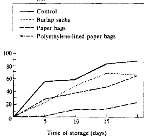
Figure 6. Effect of storage in bags on cassava (M. Col 113) root deterioration.
