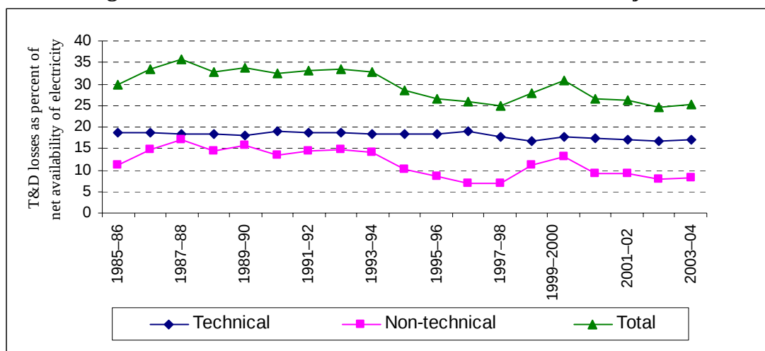
Figure 4.8: Transmission and Distribution Losses in Punjab
