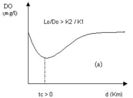
Figure 3. Relationships between DO curves and critical times, (a) t_c > 0 , (b) t_c = 0 , (c) t_c < 0
